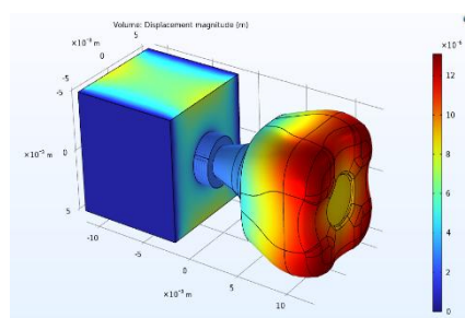
Fig.6. The displacements for 313 0 K
