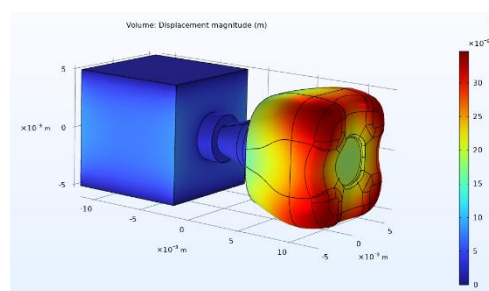
Fig.7. The displacements for 355 0 K
