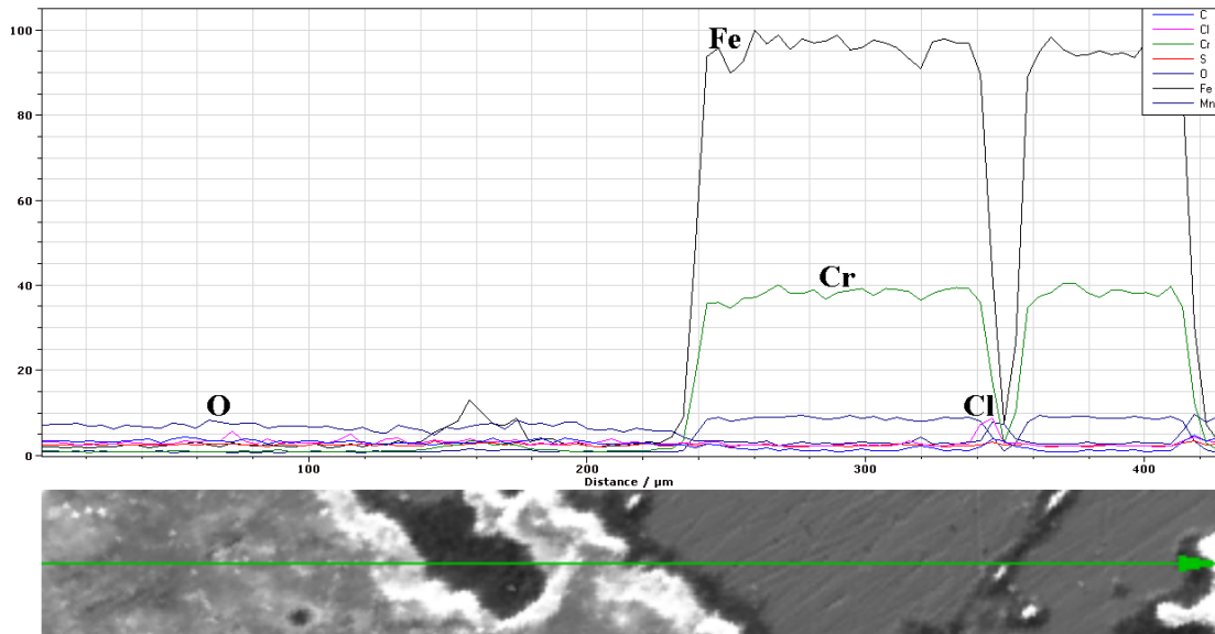
Fig. 3 The distribution of Fe, Cr, Cl and O on a corroded area on the surface of the material
